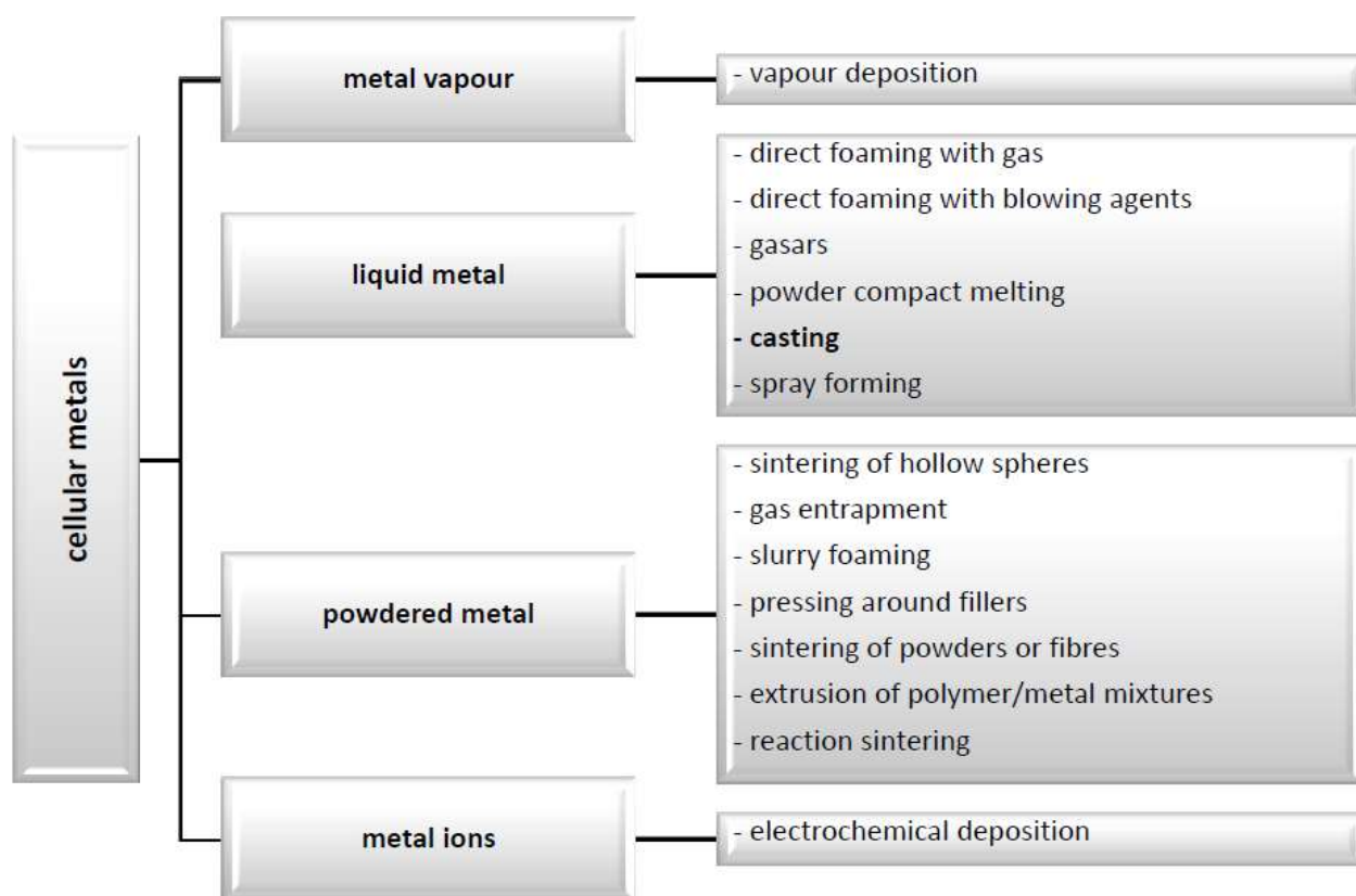
Fig. 1 Metallic foam production
