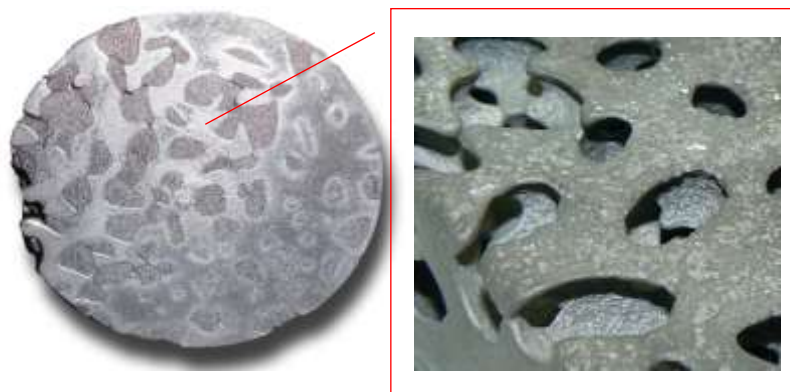
Fig. 4 Final casting and detail of its structure
