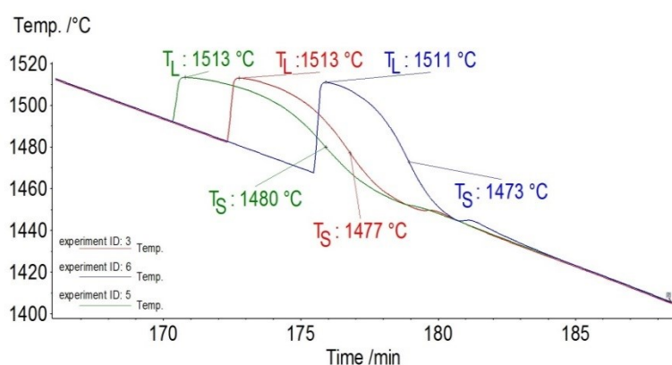
Fig.3 T_S (maximal, medium and lowest) read from individual cooling curves for studied steel grade
