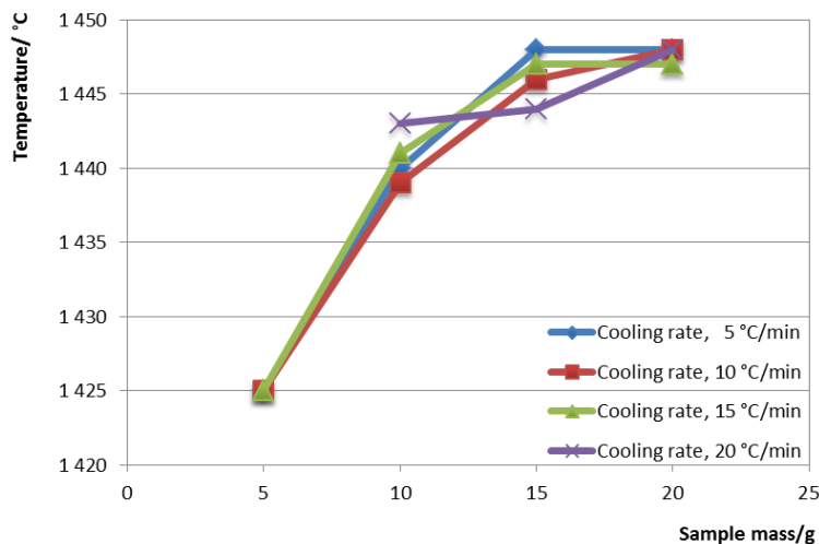
Fig.1 Nickel mass influence on the shift of solidification point temperature in mode of the linear cooling
