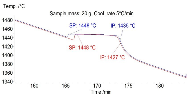
Fig.2 Similar shape of cooling curves from two experiments under the same conditions for nickel
