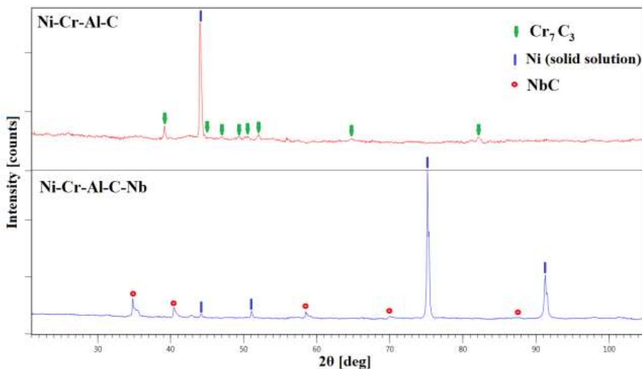
Fig. 3. XRD patterns of investigated alloys.
