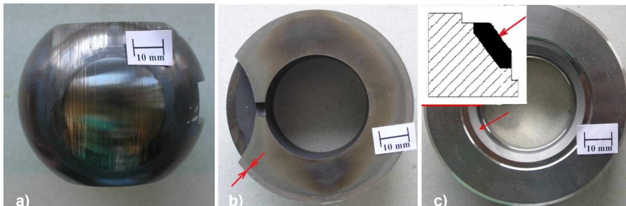
Fig. 1 Ball valves; a) - ball B – outlet side; b) - cross section of ball A cutting by electro-erosion method; c) - valve seat; Stellite welding layers are marked with red arrows
