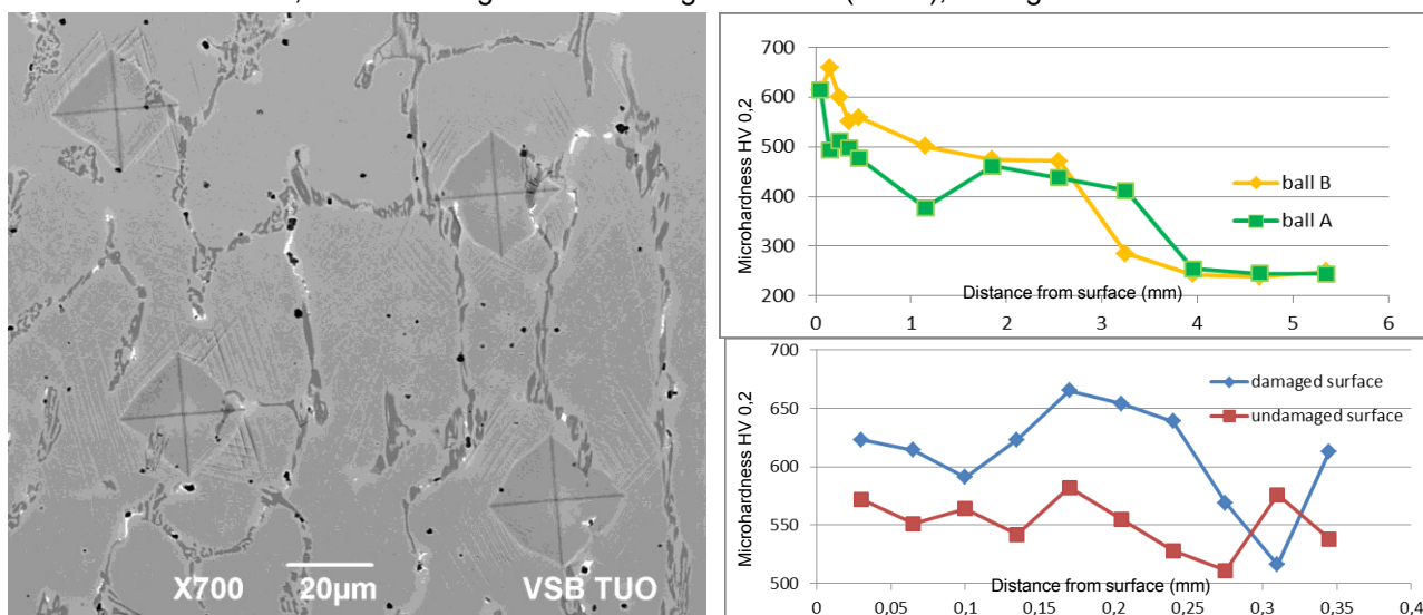
Fig. 7 Welding layer of valve seat - deformations near microindentations with cracks in eutectic phases (left); microhardness HV 0,2 of welding and buttering layer - comparison of ball A and B (above); hardness comparison of damaged and undamaged surface – ball A (below)
