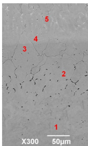
Fig. 6 The scheme of buttering layer
