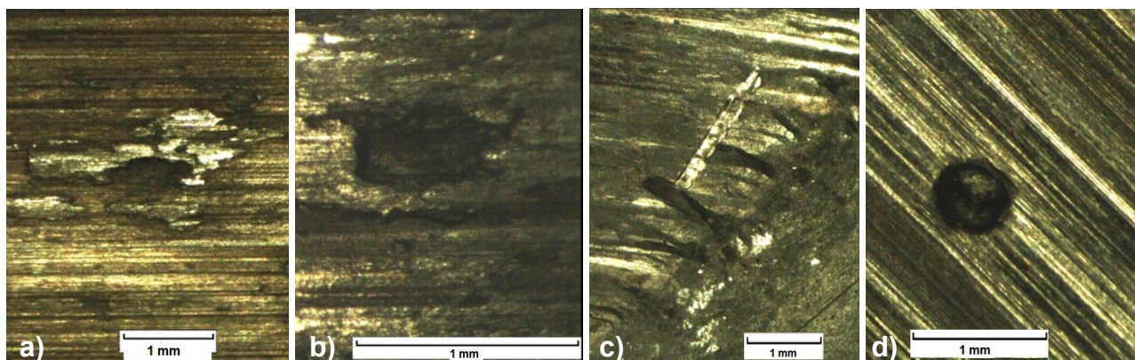
Fig. 2 Balls of ball valves – damage examples by stereomicroscope; a) – unstuck part; b) – adhesive particle; c) – damage by steam; d) – round depression
