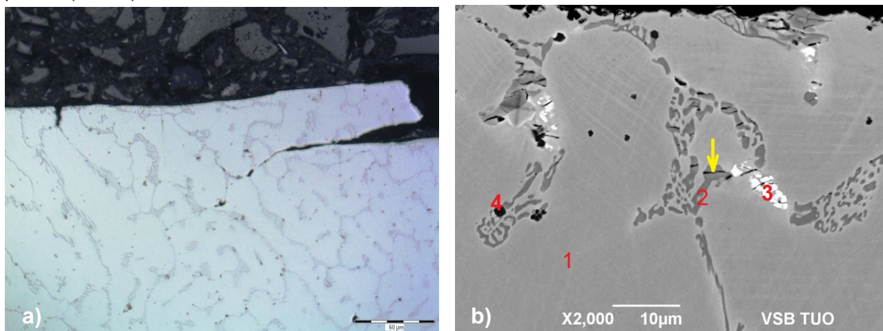
Fig. 4 Damage to the brittle structural components of seats welding layer, cracks in the eutectic phase; a) optical metallography; b) SEM analysis – the crack is marked with yellow arrow
