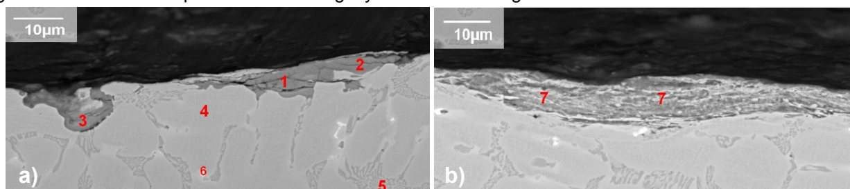
Fig. 5 Adhesive particles on the surface of Ball A
