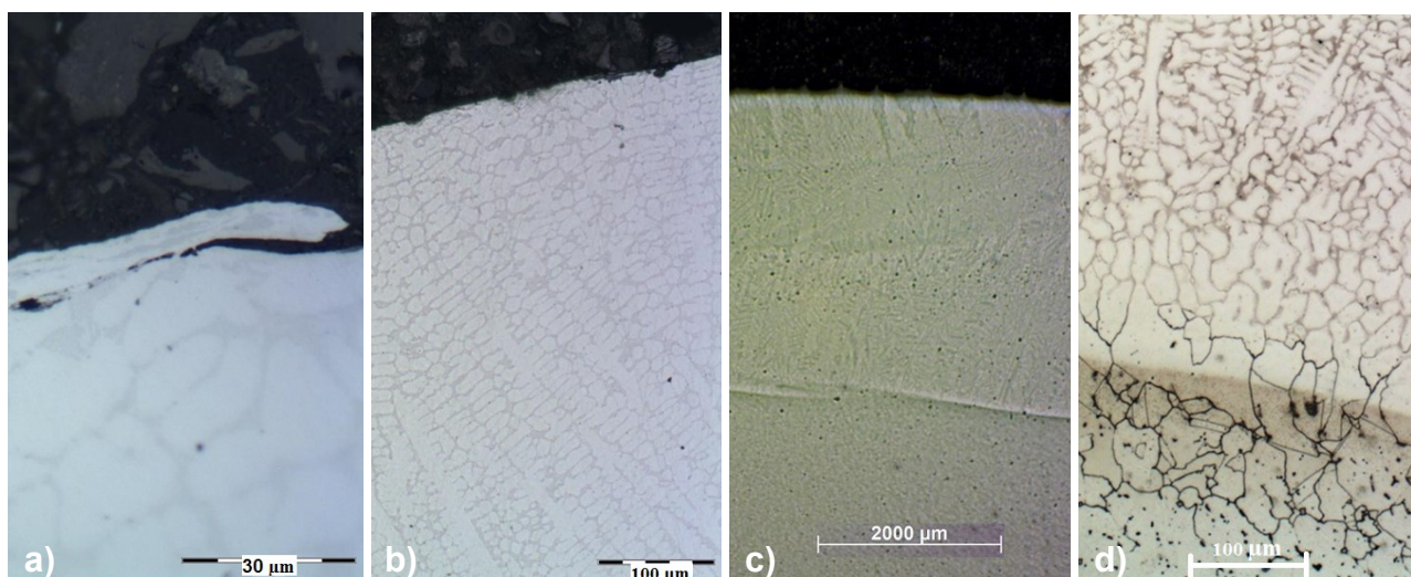
Fig. 3 Metallography of balls; a), b) – types of surface damage; c), d) – cross section of welding layer
