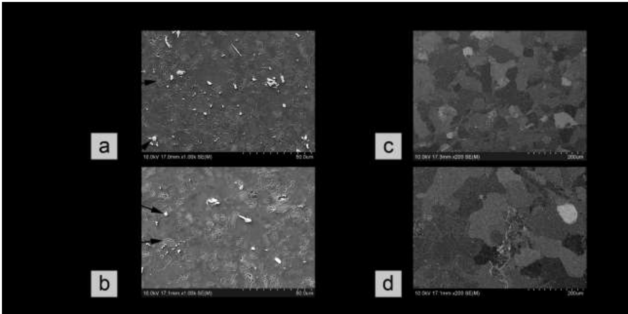
Fig.5 Microstructure of as-extruded rods from a) 413.0, \lambda=44 b) 413.0, \lambda=7 , c) 6060, \lambda=44 , d) 6060, \lambda=7 .
