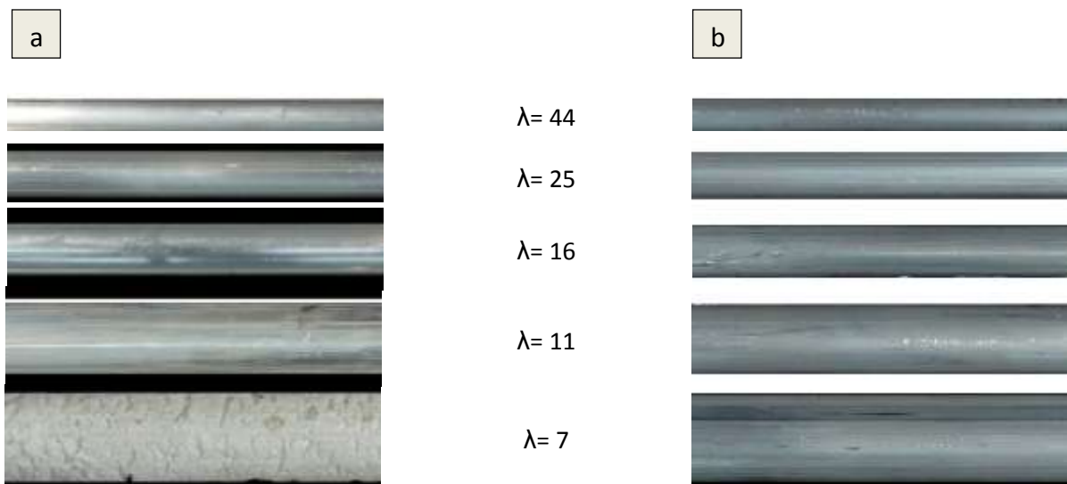
Fig. 3 Surface quality comparison of as-extruded rods from a) 413.0, b) 6060 alloy
