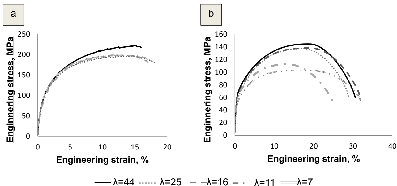
Fig. 4 Engineering stress-strain curves for a) 413.0 b) 6060 profiles.
