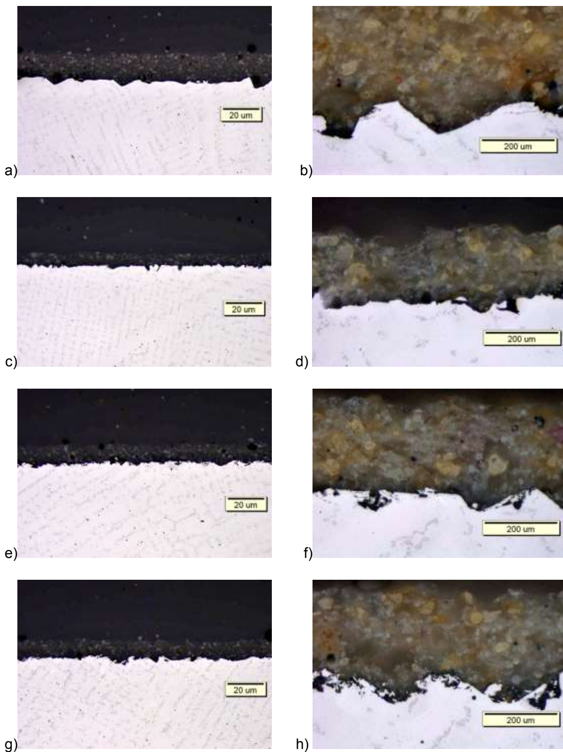
Fig. 1 The corss-section images of Ni-Cr-Mo commercial alloy coated with ceramic material. Metallic sample with sandblasted surface: a, b) 15 seconds, c, d) 1 min, e, f) 5 min, g, h) 10 min (a cross-section not etched)
