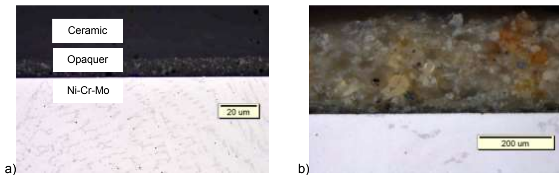
Fig. 1 The corss-section images of Ni-Cr-Mo commercial alloy coated with ceramic material – metallic sample with polished surface
