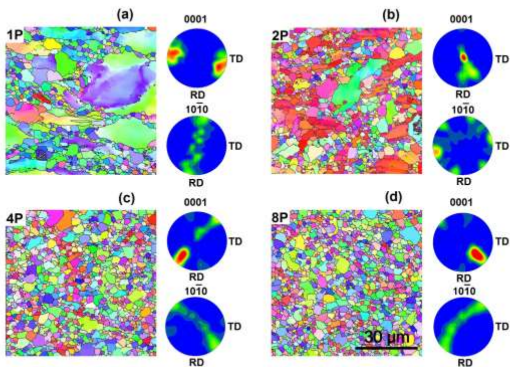
Fig. 3 Orientation maps and pole figures of TRC AZ31 magnesium alloy strip aged at 450 °C for 10 h after a) one, b) two, c) four and d) eight ECAP passes.
