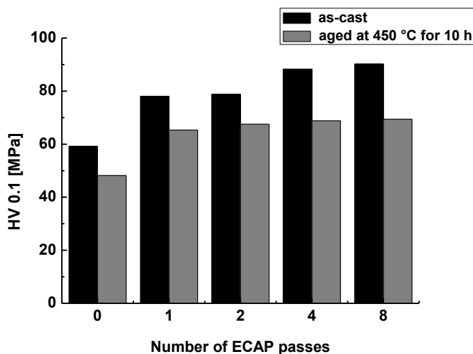
Fig. 4 Vickers microhardness (HV0.1) of the as-cast and aged at 450 °C for 10 h TRC AZ31 magnesium alloy after one, two, four and eight ECAP passes.
