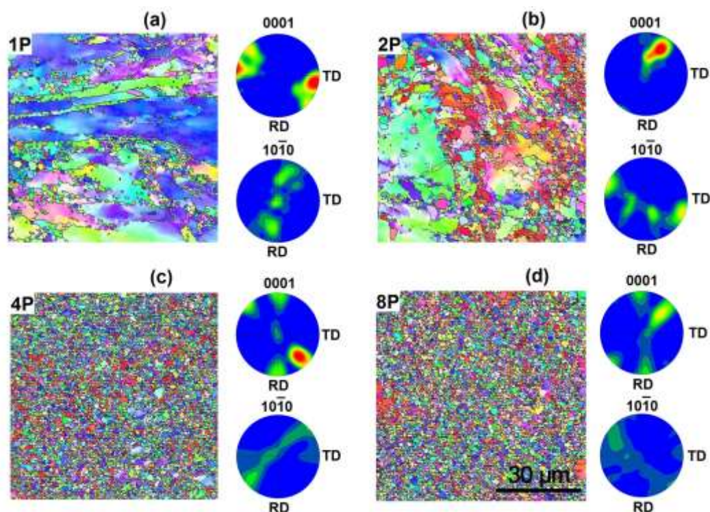
Fig. 2 Orientation maps and pole figures of as-cast TRC AZ31 magnesium alloy strip after a) one, b) two, c) four and d) eight ECAP passes.
