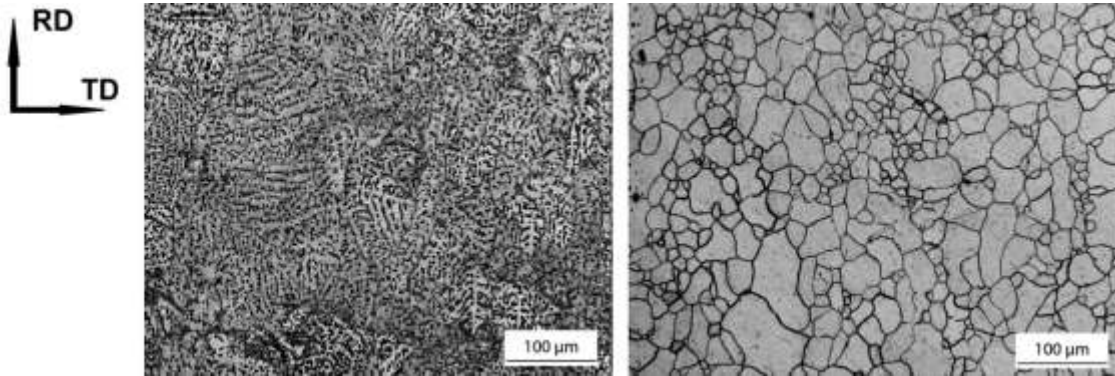
Fig. 1 Microstructure of (a) as-cast and (b) annealed (at 450 °C for 10 h) TRC AZ31 magnesium alloy strip.
