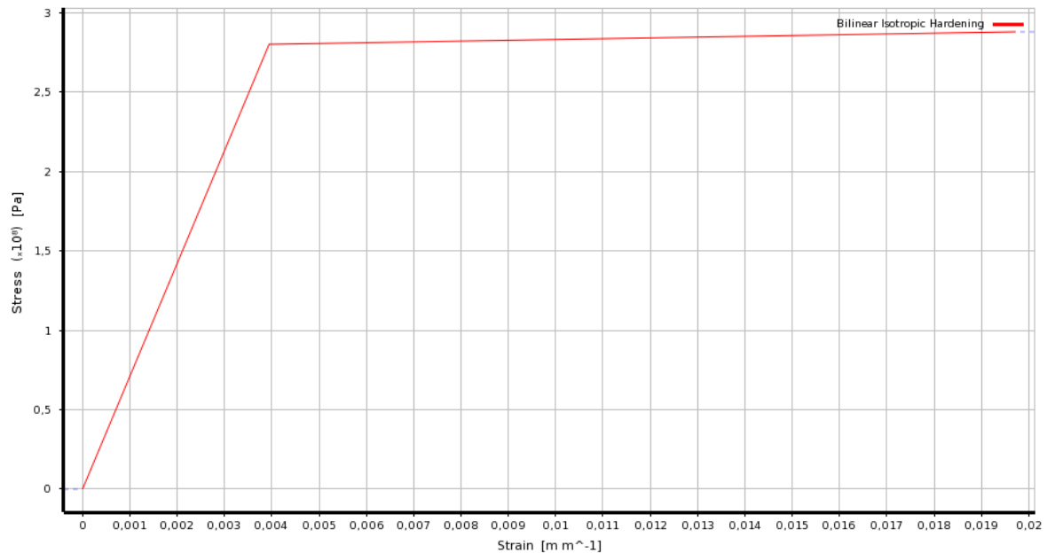
Fig. 9 Bilinear isotropic description of classical aluminum
