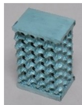
Fig. 5 The sample for the pressure test
