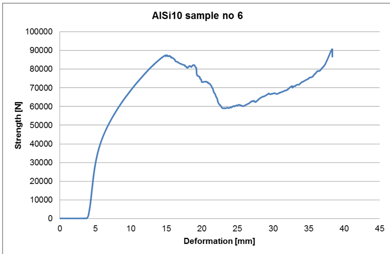
Fig. 6 The course of the pressure curve material AISI10, deformation work 2197 J
