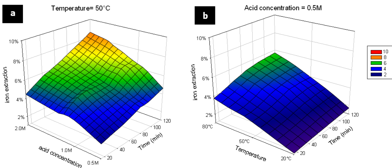
Fig. 5 Kinetic plots of iron yielded from temperature (a) and acid concentration (b)
