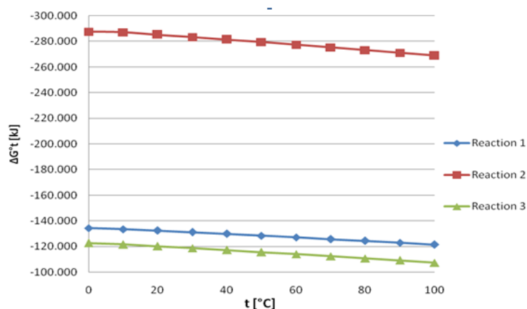
Fig. 2 Standard Gibbs energy as a function of temperature
