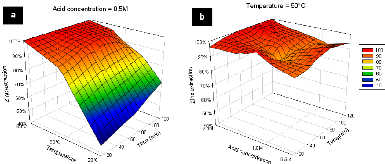
Fig. 3 Kinetic plots of zinc yielded from temperature (a) and acid concentration (b)
