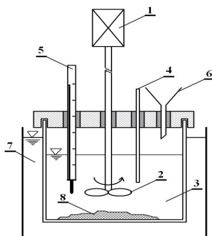
Fig. 1 Leaching apparatus [11]
