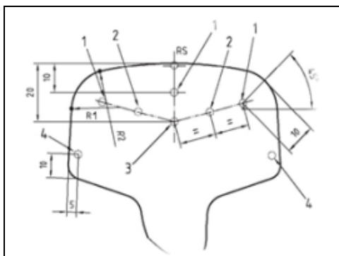
Fig. 2 Hardness regions of rails [6]
