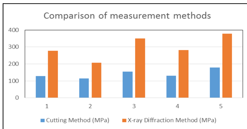
Fig. 3 Comparison between residual stress measurement methods of samples
