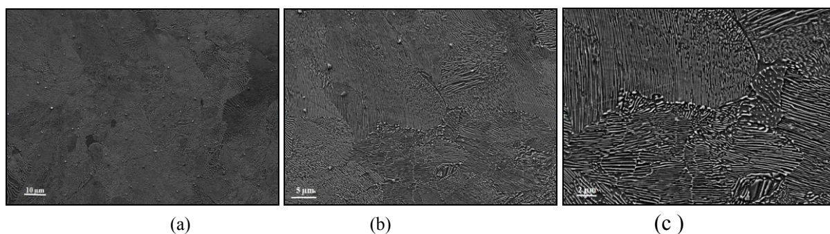
Figure 4 SEM images of rail (a) 2000X (b) 5000X (c) 10000X
