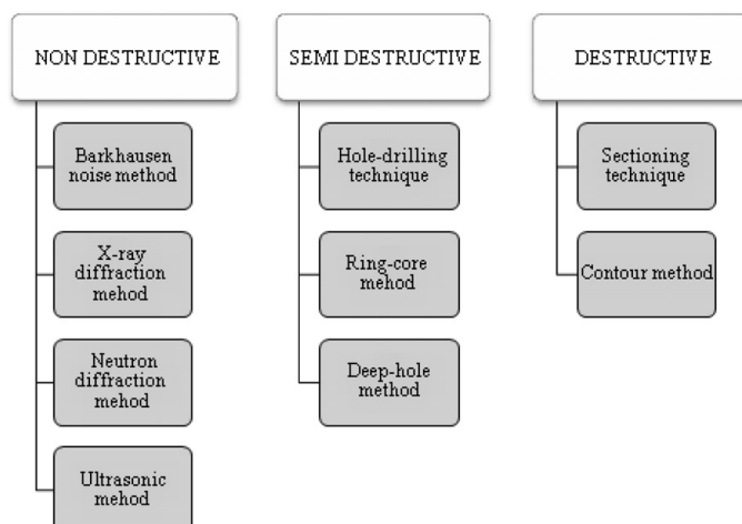
Fig. 1 Residual Stress Measurement Methods [5]
