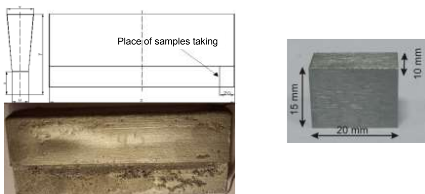
Fig. 1 Drawing of casting with the sinkhead and the appearance of the finished casting.
