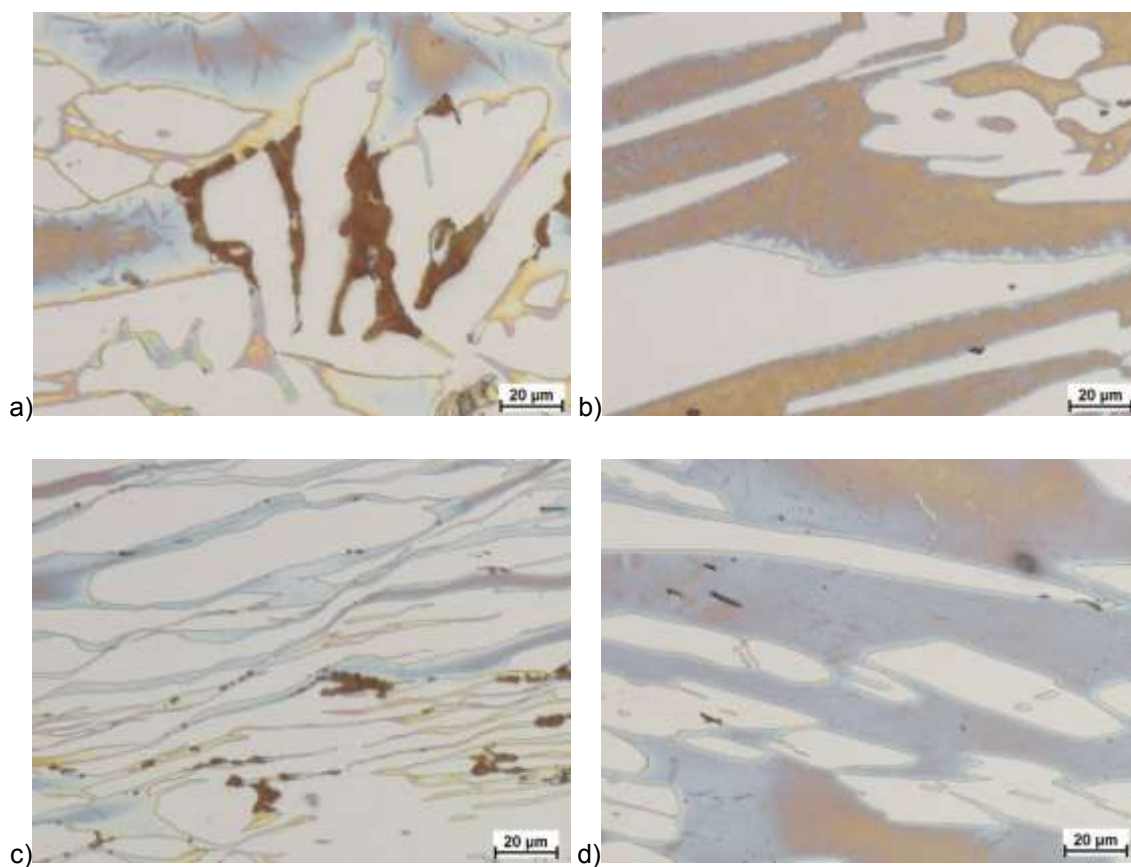
Fig. 5 Microstructure of the tested steel after deformation: a) variant 1, b) variant 2, c) variant 3, d) variant 4. mag. 500x
