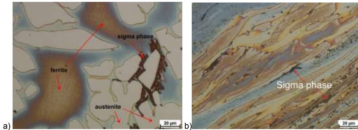
Fig. 3 Example of samples microstructures. a) Sample not deformed., b) Sample deformed sample deformed at 950°C with strain rate 1.0 and \epsilon=1.3 . magn. 500x
