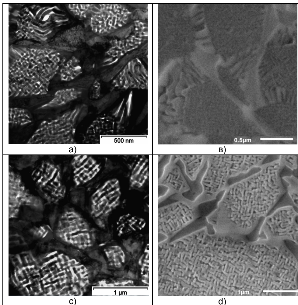
Fig. 3 (a,c) Bright-field TEM micrograph and (b,d) SEM image of the ribbon aged at 700 and 780°C
