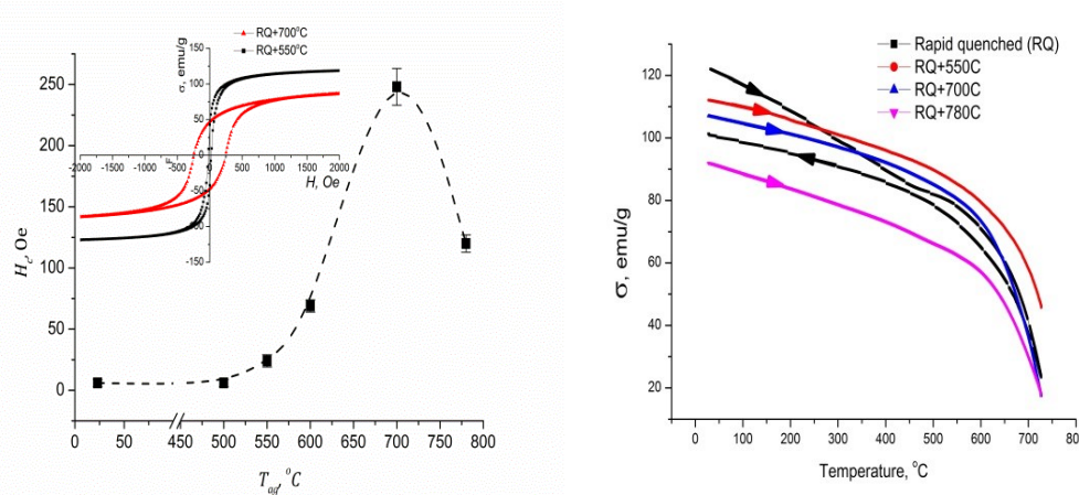
Fig. 4 Temperature dependence H_c(T_{ag}) and the hysteresis loops (inset), (b) TMA curves curve of as-prepared ribbons and the ribbons aged at 550, 700 and 780°C
