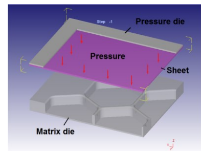
c) stamping using elastomer (hydraulic forging)
