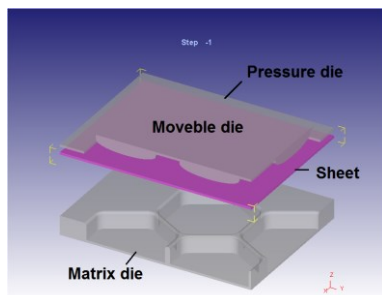
a) stretch forming (embossing). Matrix die type A
