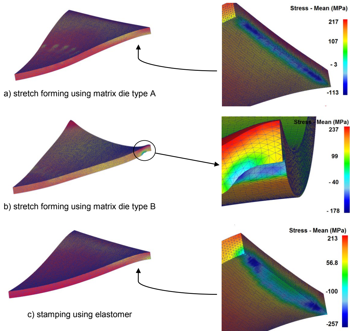
Fig. 4 Distribution of maximal internal stresses in the body of a sheet
