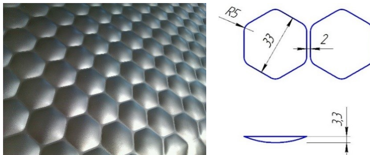
Fig. 1 Structured sheet and its geometric characteristics (in mm)
