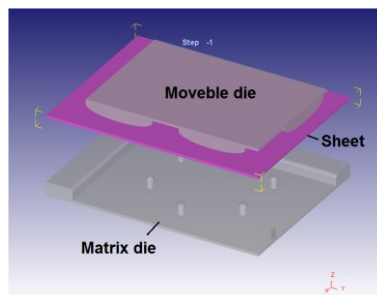
b) stretch forming (embossing). Matrix die type B
