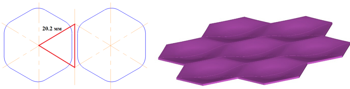
Fig. 3 Geometric shape of the single element of structured sheet. The red paint shows the element of structured sheet which reflection allows to repeat the shape of the whole structured sheet entirely
