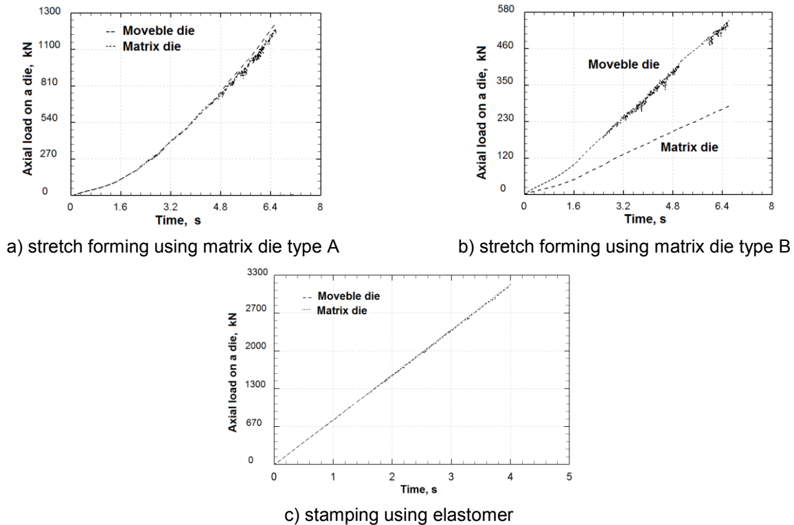
Fig. 5 Axial load on a die by production of structured sheet dimensions 500 x 500 mm
