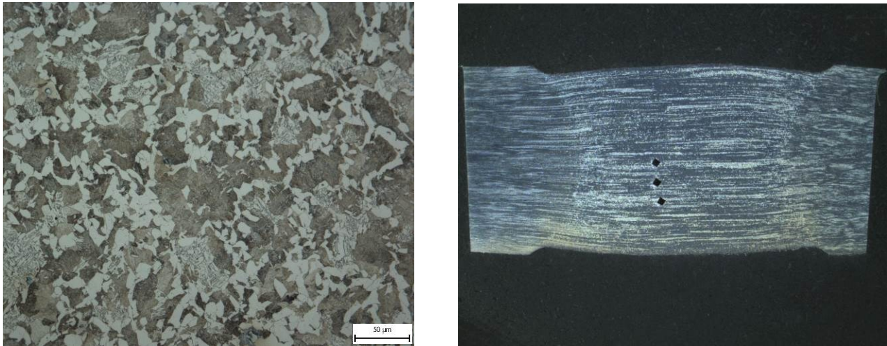
Fig. 4 Left: microstructure of the modelling specimen replicating the P7 point after cooling still in air – K0 cooling curve. Right: macrostructure on the cross-section through the modelling specimen
