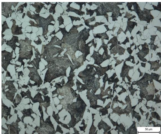
Fig. 8 Left: microstructure of the modelling specimen replicating the P7 point – controlled cooling according to K3 cooling curve. Right: macrostructure on the cross-section through the modelling specimen
