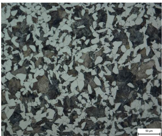
Fig. 9 Left: microstructure of the modelling specimen replicating the P7 point – controlled cooling according to K4 cooling curve. Right: macrostructure on the cross-section through the modelling specimen
