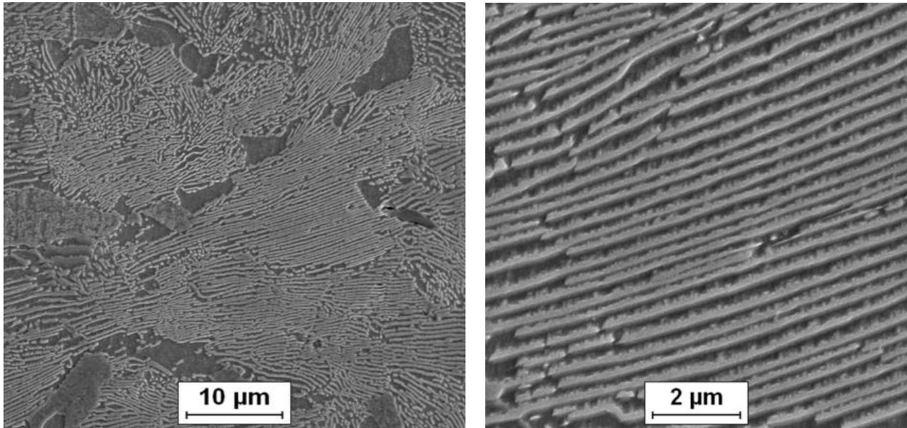
Fig. 3. Microstructure of C70D grade steel colled after deformation steps with cooling rate 1°C / s
