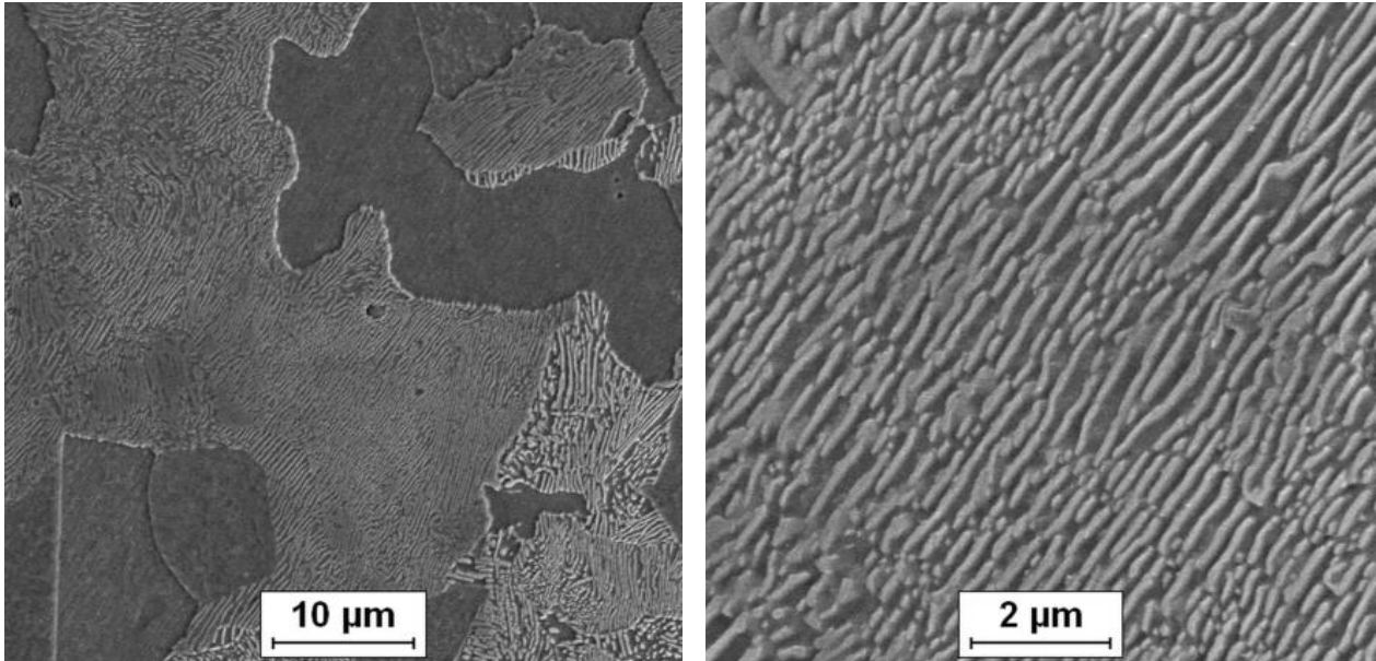
Fig. 2. Microstructure of C46D grade steel cooled after deformation steps with cooling rate 1°C / s
