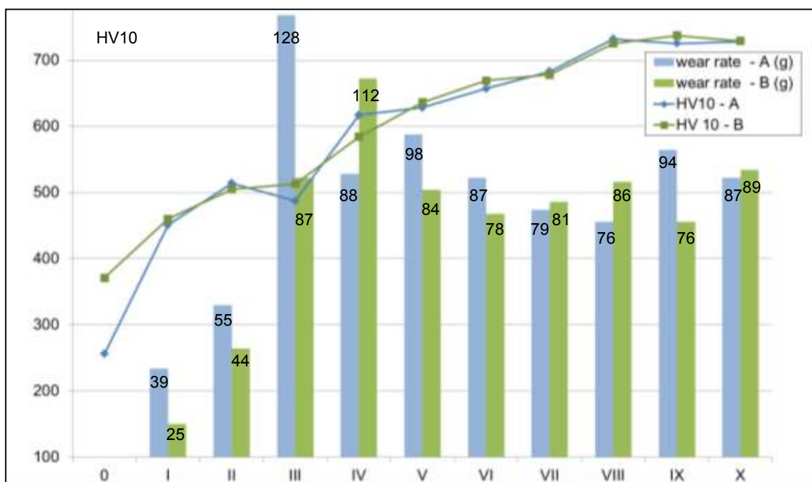
Fig.2 Hardening process vs. wear rate induced by experimental contact loading, in HV10 values (A...samples without explosive hardening, B... samples after explosive hardening)
