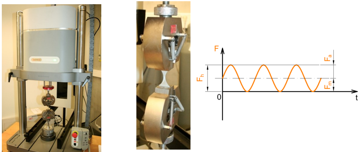
Fig. 5 Machine for cyclic tests Instron E3000 and chosen loading cycle
