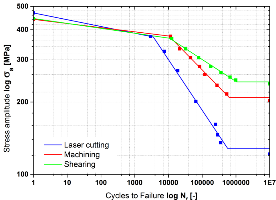
Fig. 8 Wöhler's curves of TRIP steel RA-K 40/70 for different material cutting technologies
