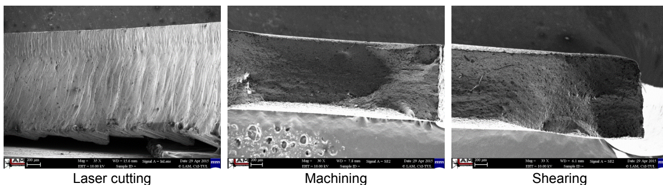
Fig. 7 Images of fatigue failure surfaces loaded by transient cycle with amplitude of stress 325 MPa
