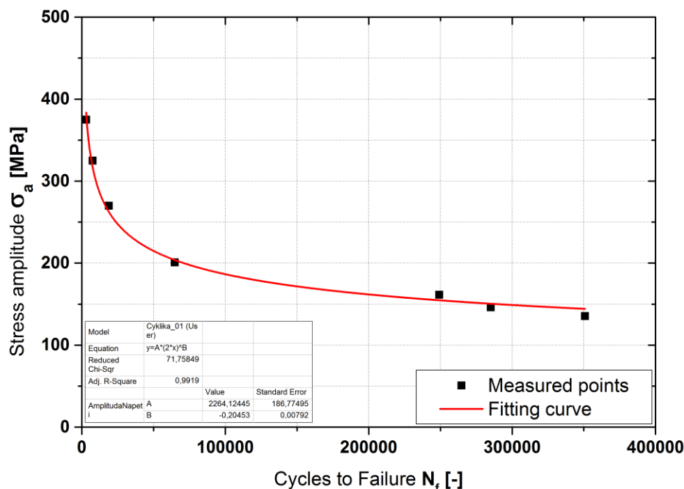
Fig. 6 Example of computation approximation constants for the laser cutting technology
