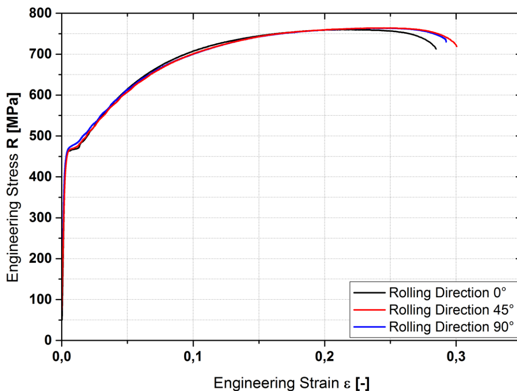
Fig. 2 Results from the static tensile test – material: RA-K 40/70
