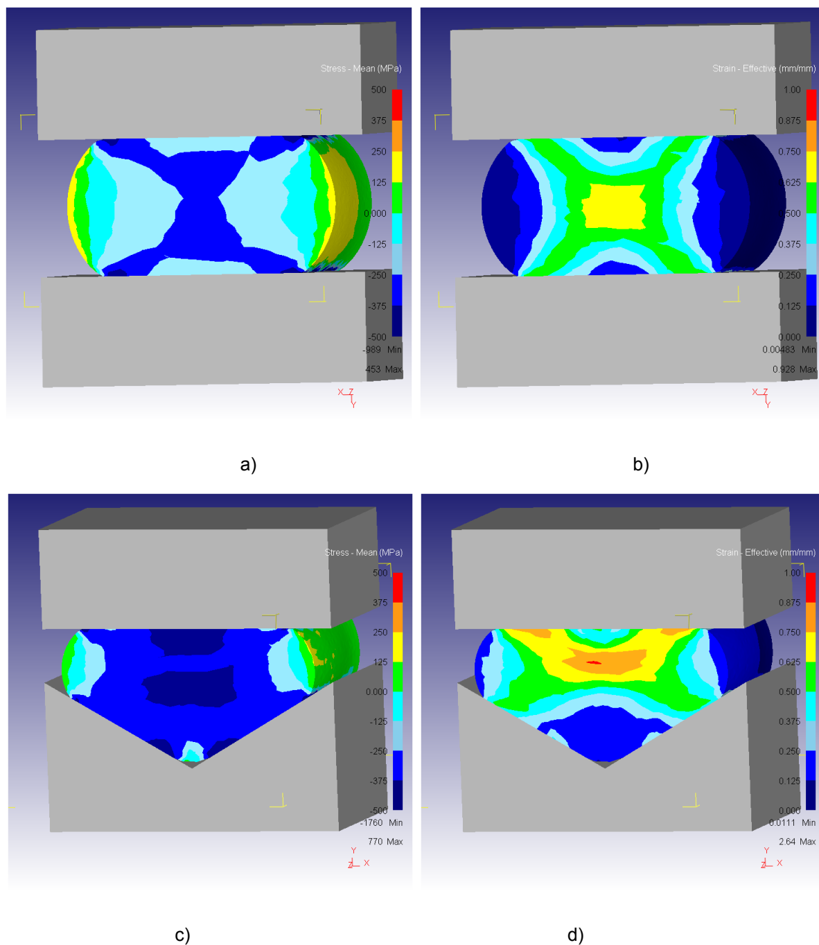
Fig.1. Distribution stress mean (a, c) and strain effective (b, d) by cross section during fullering in flat dies (a, b) and combined dies (c, d)
