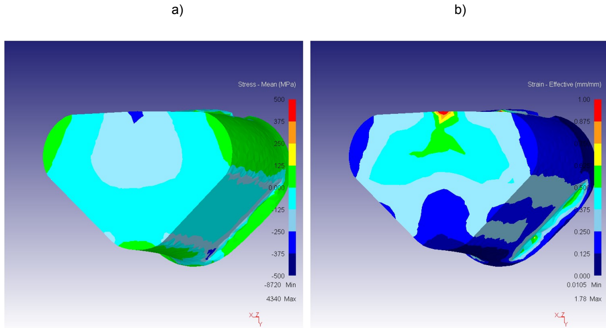
Fig.2. Distribution stress mean (a) and strain effective (b) by cross section during fullering in new dies
