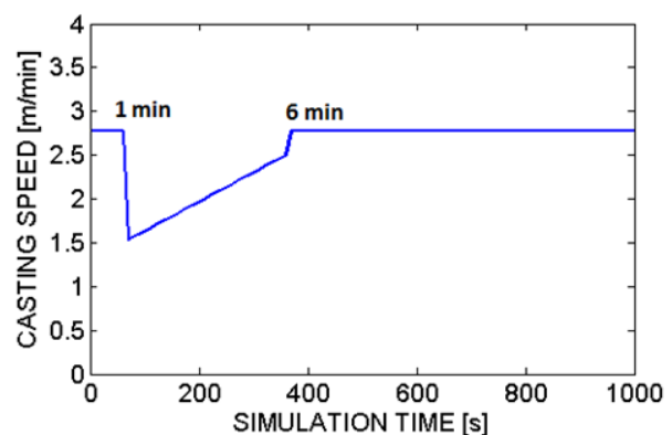
Fig. 2 Casting speed for the study case
