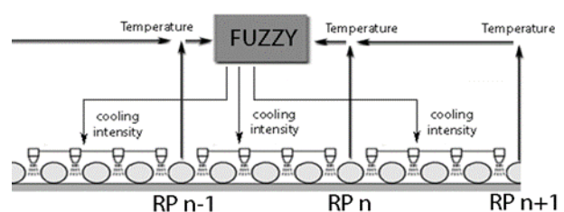
b) Fuzzy control system in secondary cooling
