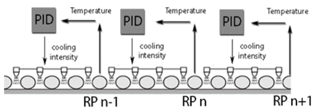
a) PID regulation of secondary cooling
