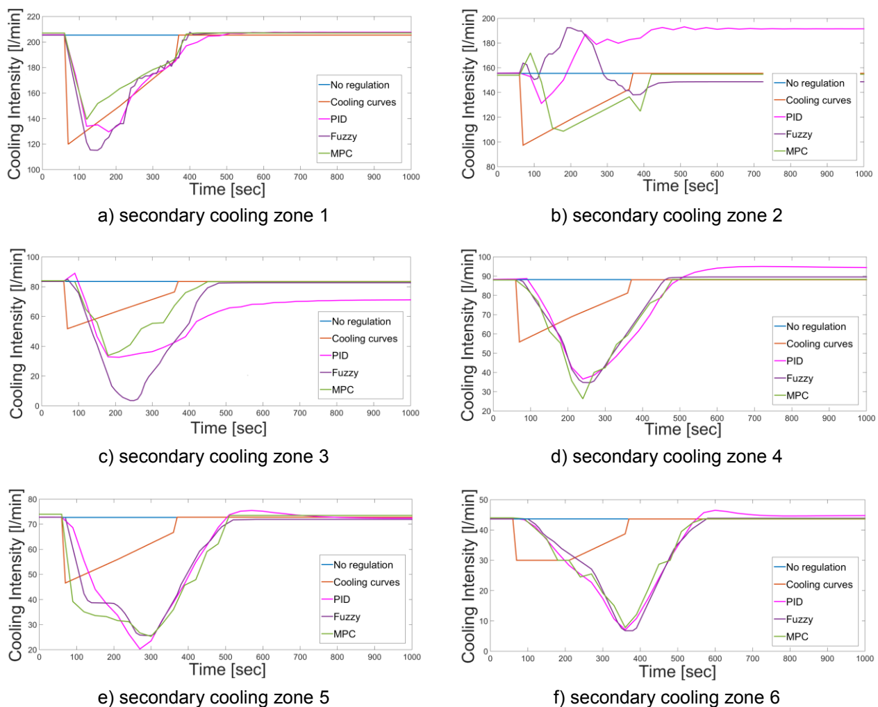
Fig. 4 Water flow rates in secondary cooling zones determined by means of distinct control approaches
