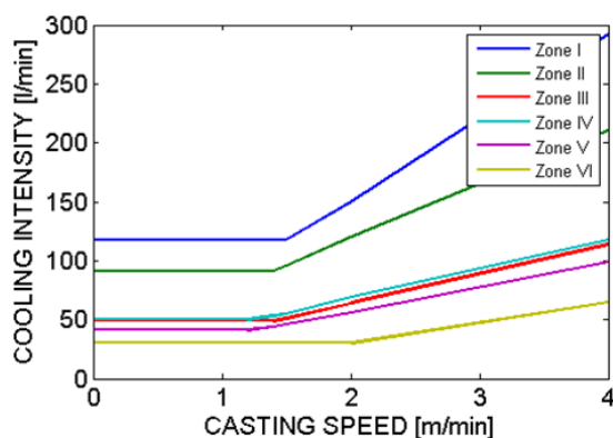
Fig. 1 Cooling curves
