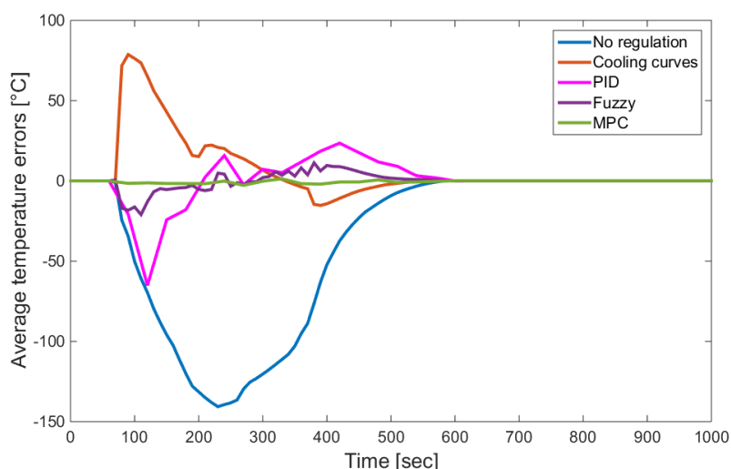
Fig. 5 Average surface temperature errors for distinct regulation approaches
