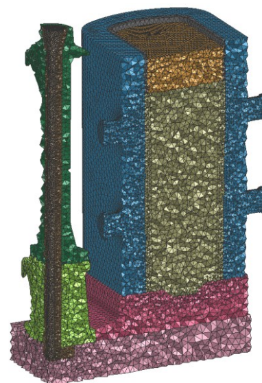
Fig.2 View of the final computational mesh of the casting system
