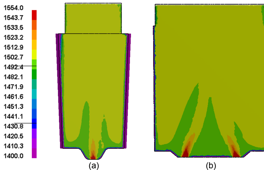
Fig.4 Comparison of the temperature field (in °C) at the end of filling in the cross section of the classical conventional polygonal ingot (a) and slab ingot (b)
