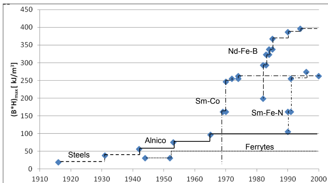
Fig. 3 Examples of the permanent magnets manufactured on an industrial scale over the last century with the increasing value of the magnetic energy density (BH)_{\max} , as the measure of their magnetic quality.
