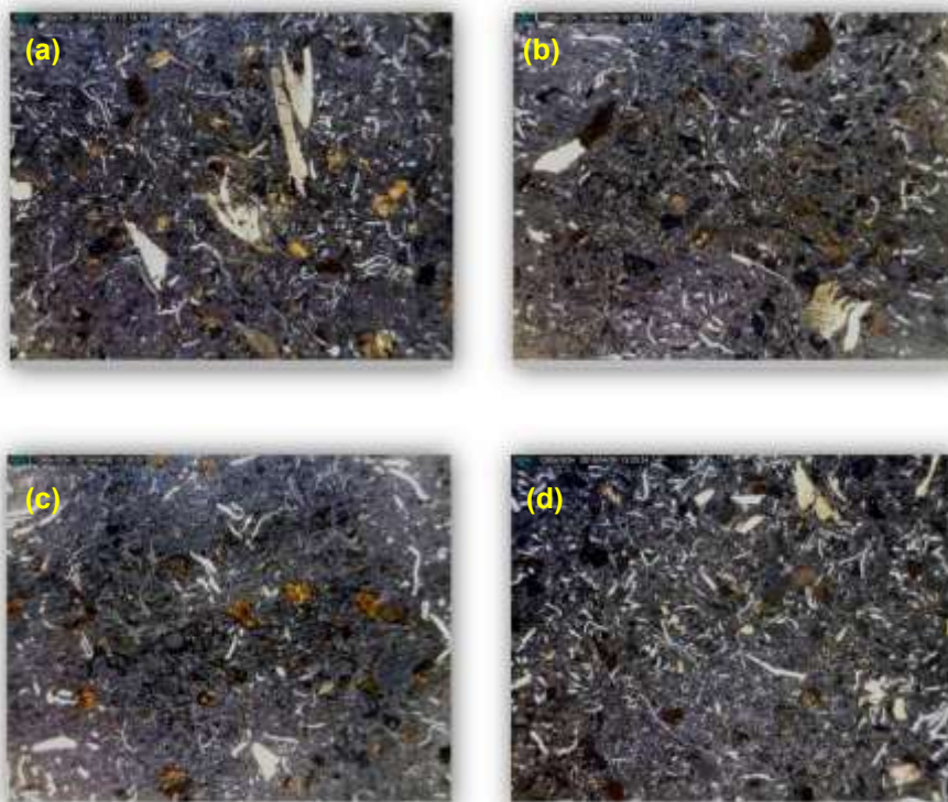
Fig. 6 The microstructure of brake pads with natural dusts: a) 1A b) 1B c) 2A d) 2B
