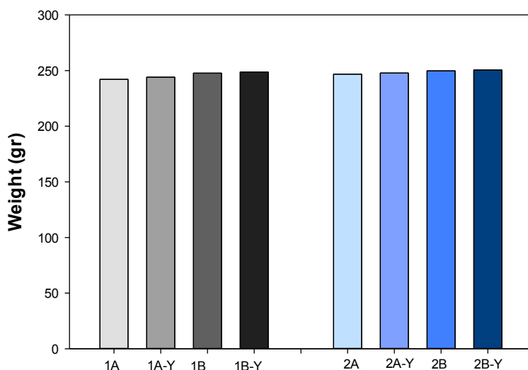
Fig. 8 The weight variations of brake pads with hazelnut and walnut (3.5 % and 7 %)
