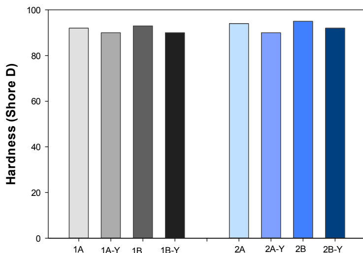
Fig. 7 The hardness variations of brake pads with hazelnut and walnut (3.5 % and 7 %)
